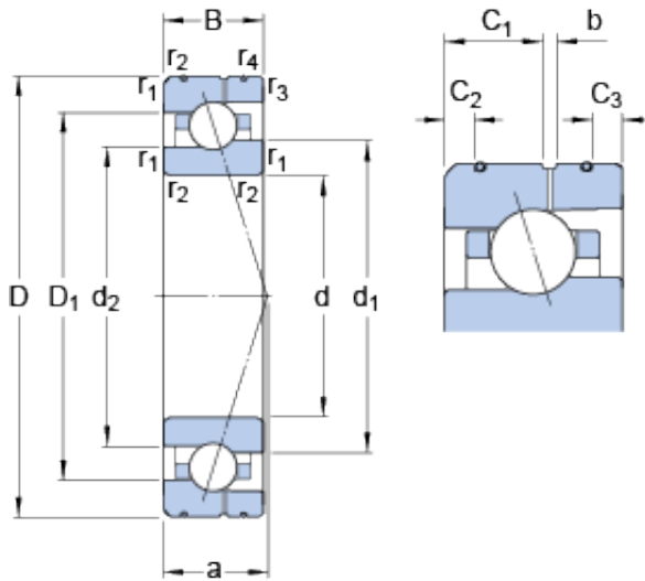
Bearing No. 7007 ACE/P4AL
