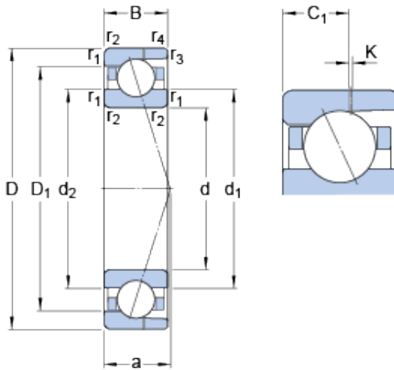
Bearing No. 7008 ACD/P4AH
