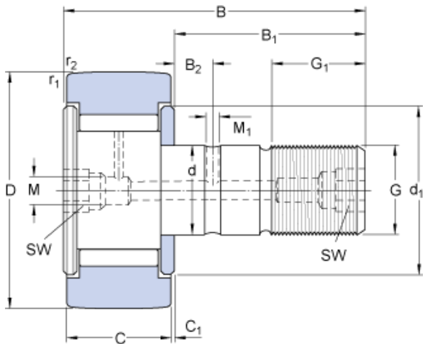
Bearing No. KRV 30 B
