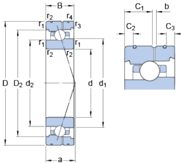
Bearing No. 7009 ACB/P4AL
