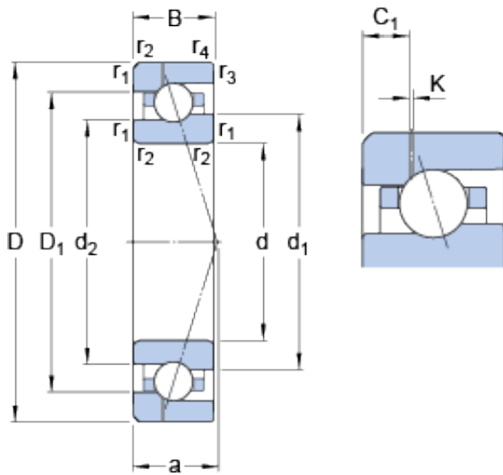
Bearing No. 7009 ACE/HCP4AH1
