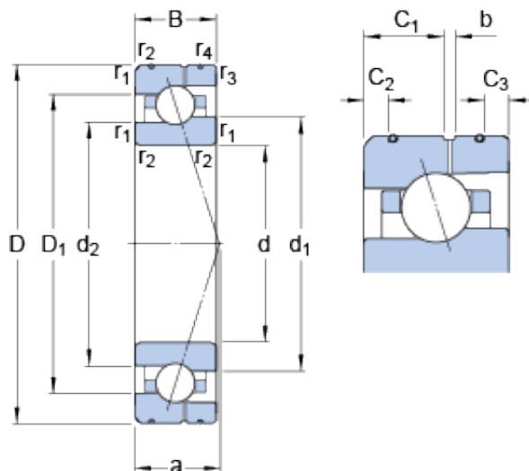
Bearing No. 7009 ACE/HCP4AL
