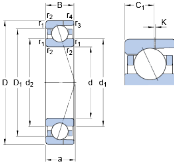
Bearing No. 7009 CD/HCP4AH
