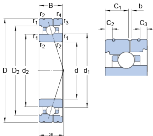
Bearing No. 7010 ACB/P4AL
