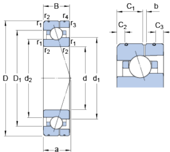
Bearing No. 7010 ACE/P4AL
