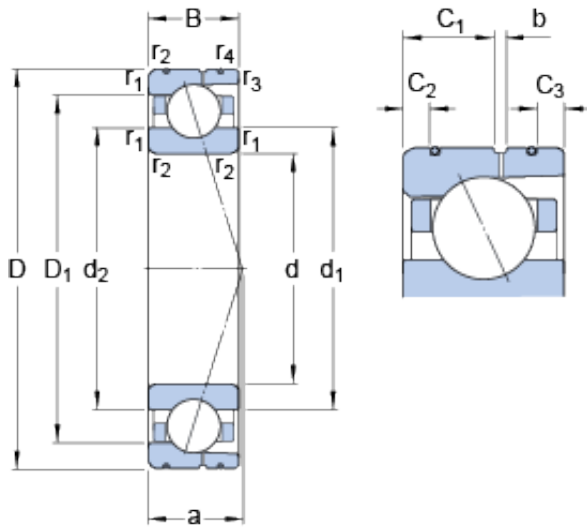
Bearing No. 7010 CD/P4AL
