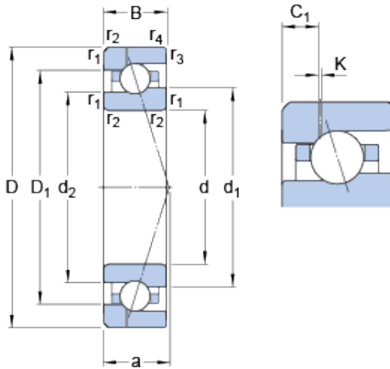
Bearing No. 7010 CE/P4AH1
