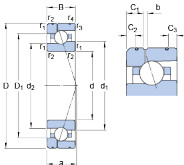
Bearing No. 7010 CE/P4AL1
