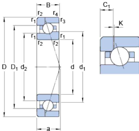
Bearing No. 7019 ACE/HCP4AH1
