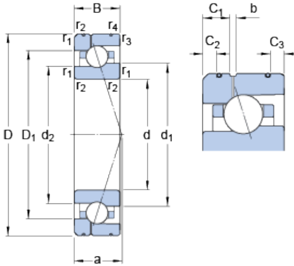
Bearing No. 7019 ACE/HCP4AL1
