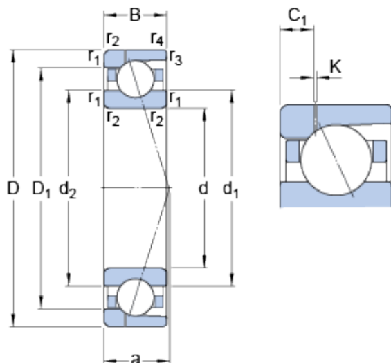
Bearing No. 7019 CD/P4AH1
