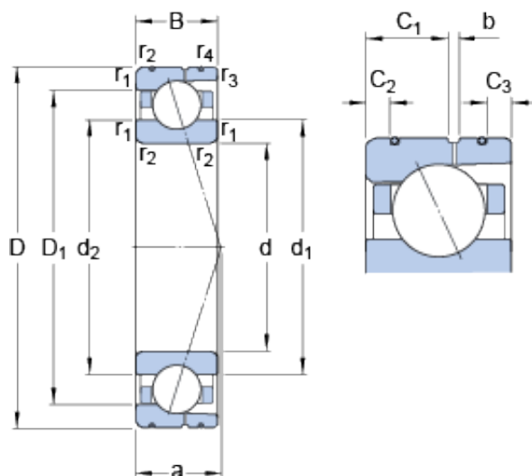
Bearing No. 7026 ACD/P4AL
