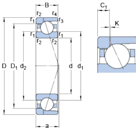
Bearing No. 7026 CD/P4AH1
