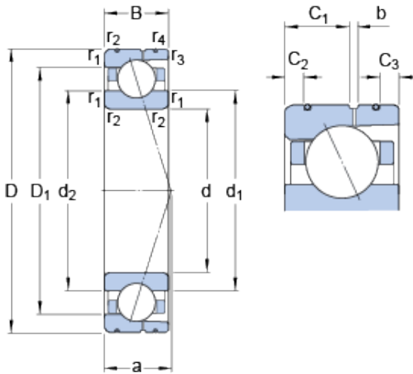
Bearing No. 7026 CD/P4AL
