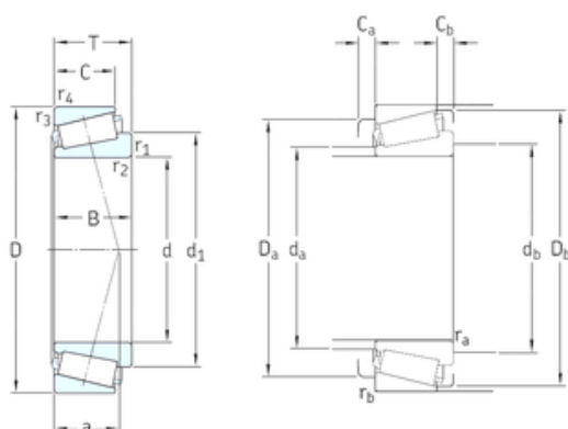
Bearing No. 32303J2/Q
