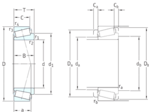
Bearing No. 32310BJ2/QCL7C
