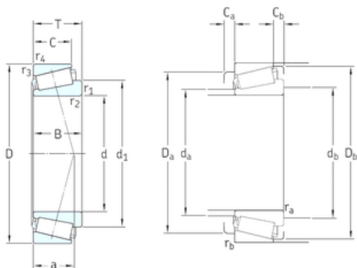
Bearing No. 32313BJ2/QU4CL7CVQ267
