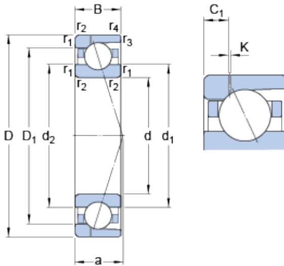
Bearing No. 7038 CD/P4AH1
