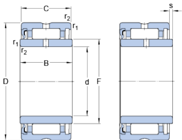
Bearing No. NA 4904 RS
