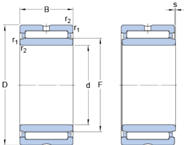
Bearing No. NA 4906
