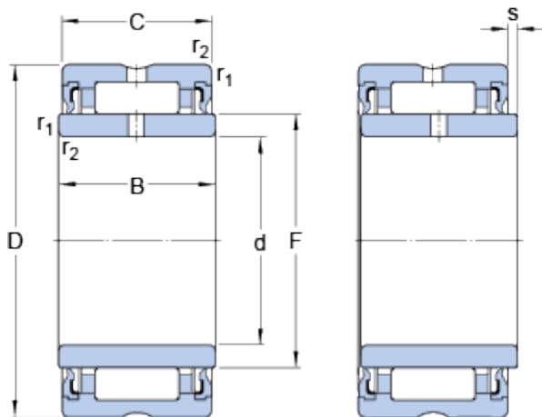
Bearing No. NA 4907.2RS
