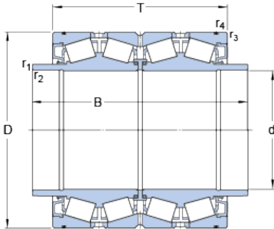
Bearing No. BT4B 328223 G/HA1VA901
