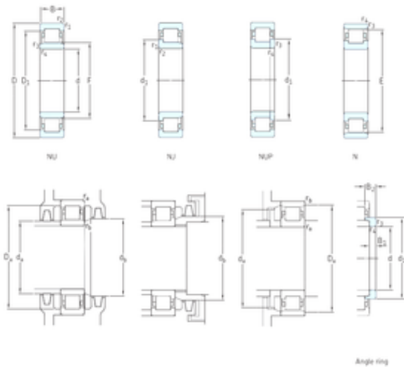
Bearing No. NU1088MA
