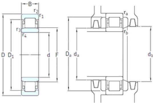
Bearing No. NU1012M/HC5C3
