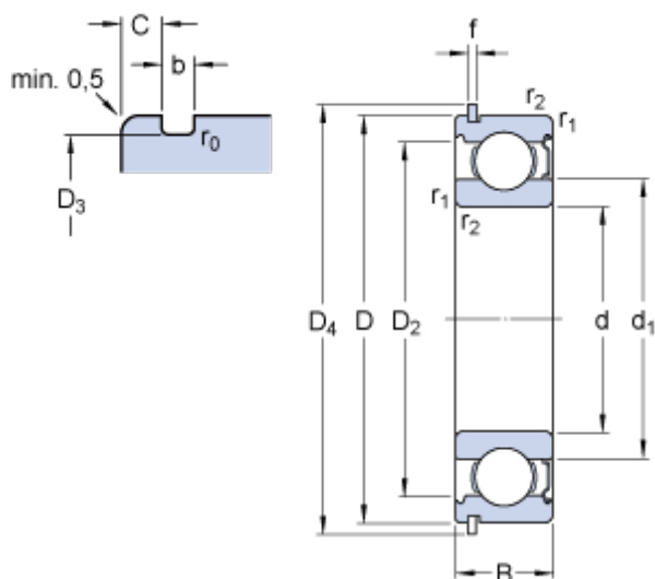
Bearing No. 6203-ZNR
