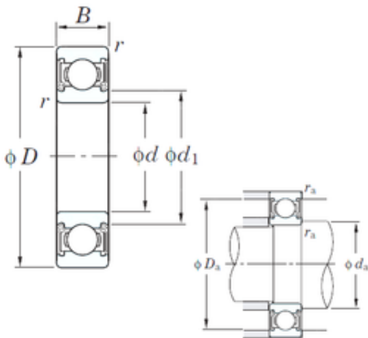
Bearing No. 6207 2RD C3
