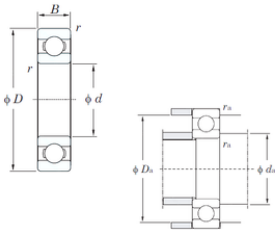
Bearing No. 6207R
