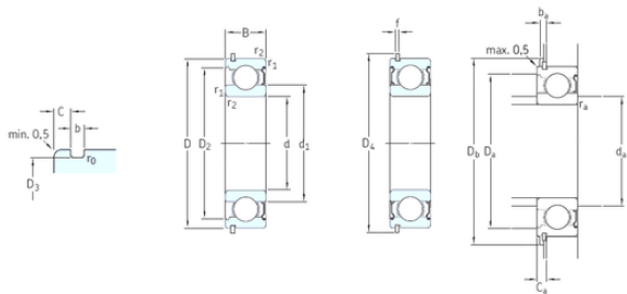
Bearing No. 6209-2ZNR
