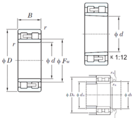
Bearing No. NNU4964K
