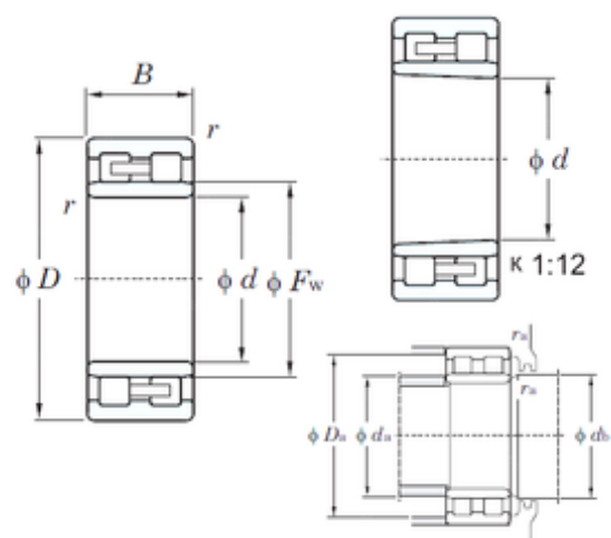
Bearing No. NNU4956K
