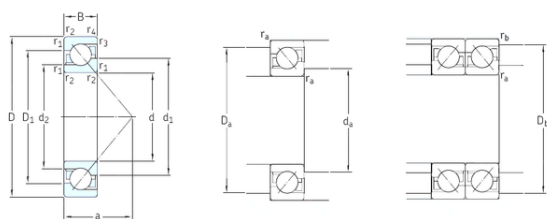
Bearing No. 7314BEGAPH
