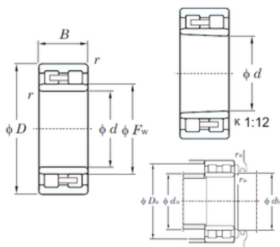
Bearing No. NNU4934K
