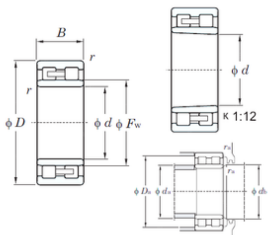
Bearing No. NNU4921
