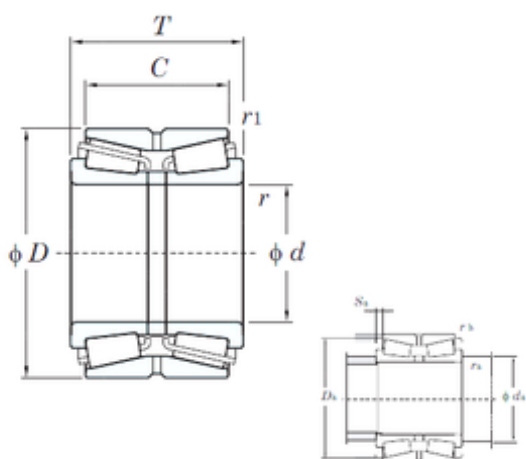
Bearing No. 46372A
