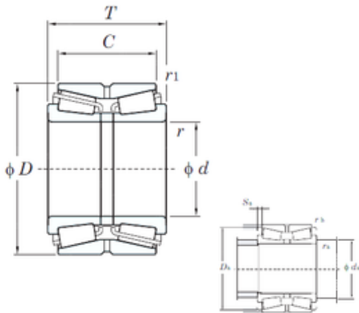
Bearing No. 46T30317JR/77
