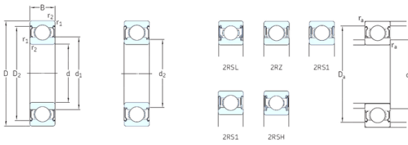
Bearing No. E2.6307-2Z
