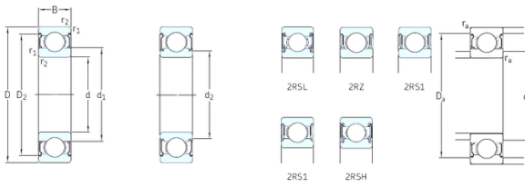
Bearing No. 62300-2RS1
