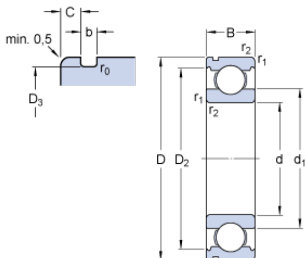
Bearing No. 6303 N
