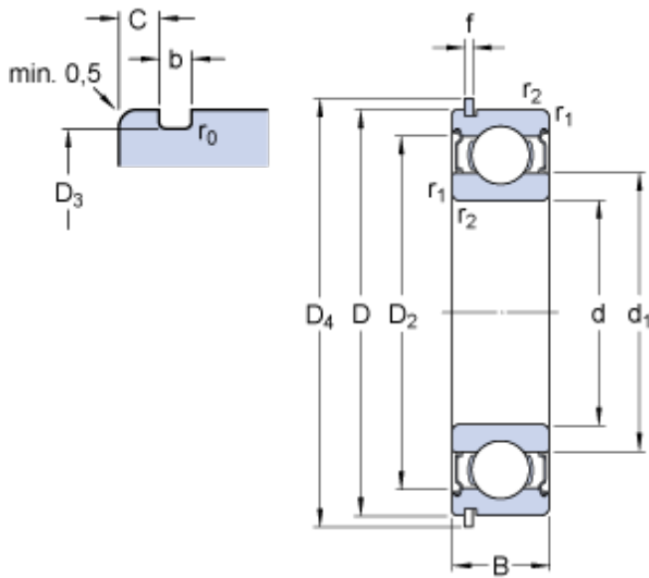
Bearing No. 6303-2ZNR
