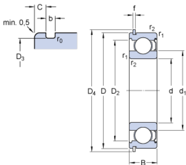
Bearing No. 6303-ZNR
