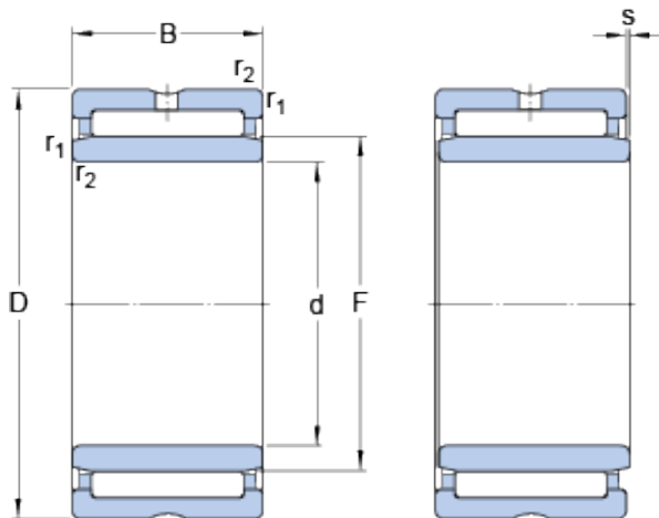
Bearing No. NKIS 55
