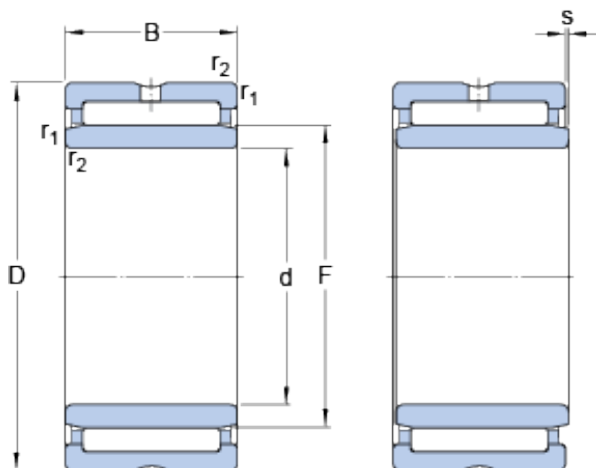
Bearing No. NKI 70/35
