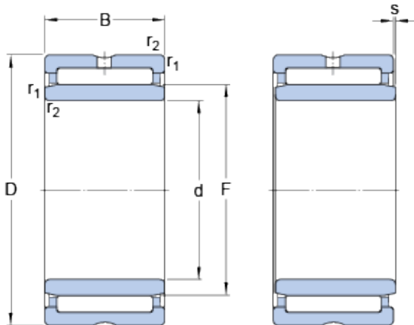
Bearing No. NKI 85/26
