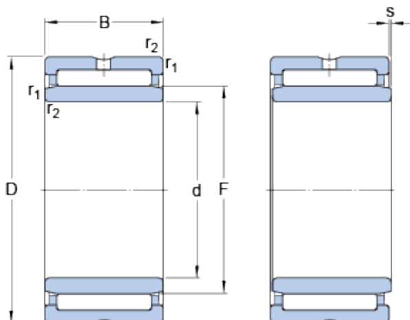
Bearing No. NKI 25/20 TN
