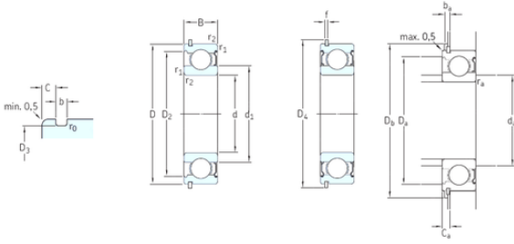
Bearing No. 6308-2ZNR
