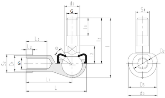
Bearing No. SQYL7-RS
